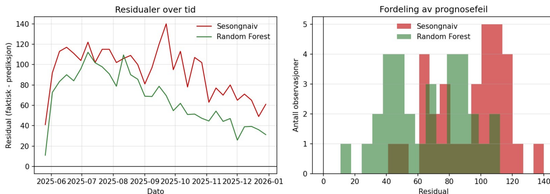
Figur 6.4: Residualanalyse
